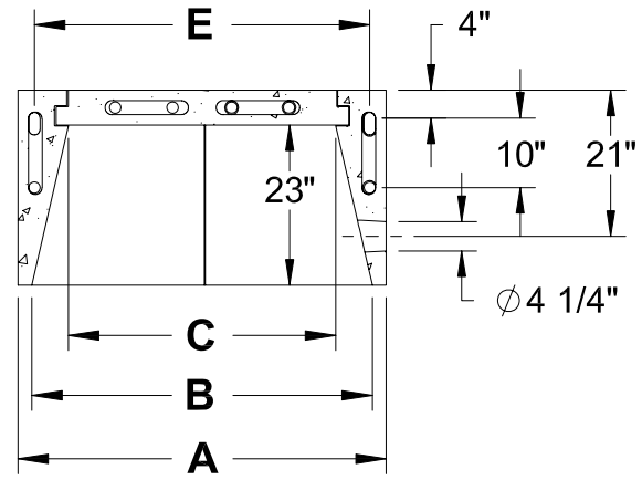
SECTION G-G
